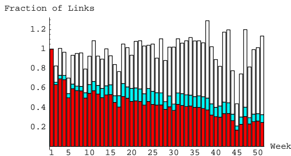
Figure 7: Normalized fraction of shingles from the first crawl still existing after n weeks (dark portion of bars) and shingles newly created (light portion).
