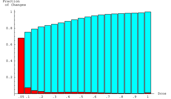
Figure 11: Distribution of cosine distance for all changes. Each dark bar corresponds to changes with cosine distance between the respective x-axis value and the previous one. For example, bin 0.1 corresponds to changes with cosine distance between 0.05 and 0.1. The light bars show the cumulative distribution.
